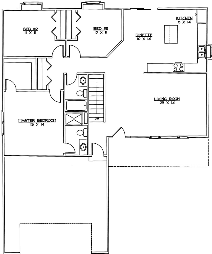
MAIN FLOOR - 1396 through 1448 Sq. Ft.
