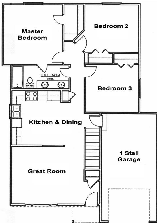
MAIN FLOOR - 1147 Sq. Ft.
