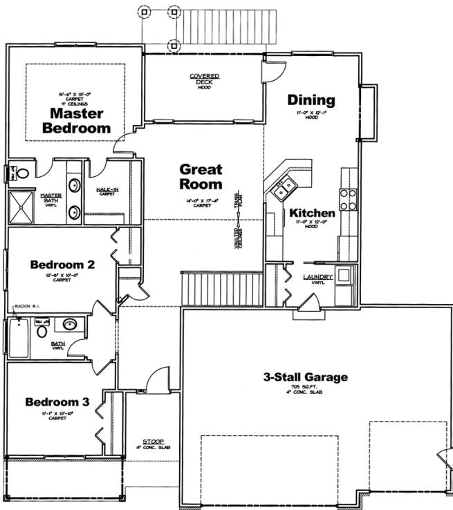
MAIN FLOOR - 1465 Sq. Ft.
