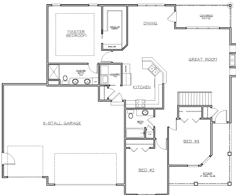
MAIN FLOOR - 1567 Sq. Ft.
