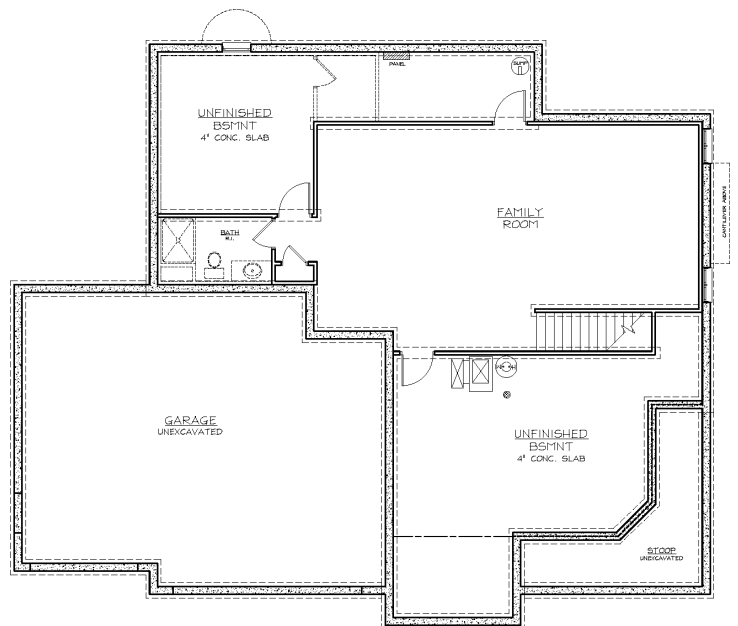
BASEMENT - 1567 Sq. Ft.
