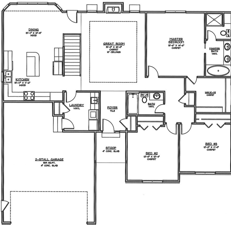
MAIN FLOOR - 1704 Sq. Ft.
