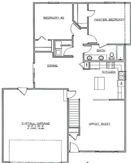
MAIN FLOOR - 1175 Sq. Ft.
