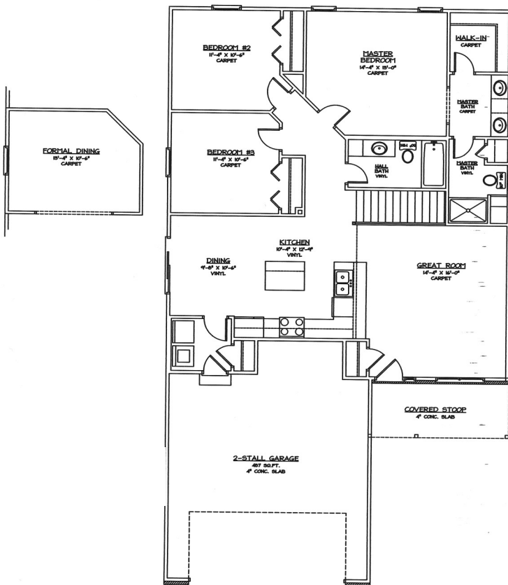
MAIN FLOOR - 1375 Sq. Ft.
