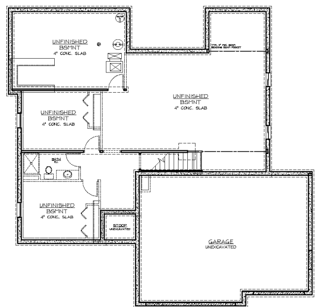
BASEMENT - 1547 Sq. Ft.
